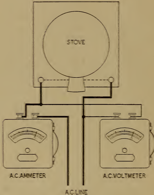
FIG. 15.—EFFICIENCY TEST OF AN ELECTRIC DISK STOVE OR HOT PLATE. (Reproduced from Students' Sketch.) Philippi's Method.
